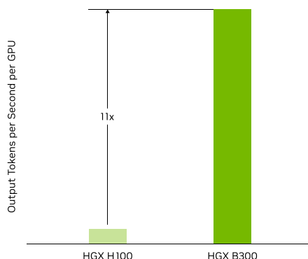
Llama 3.1 405B Real-Time Throughput
